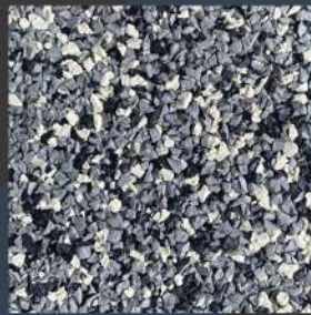
QUARTZ
